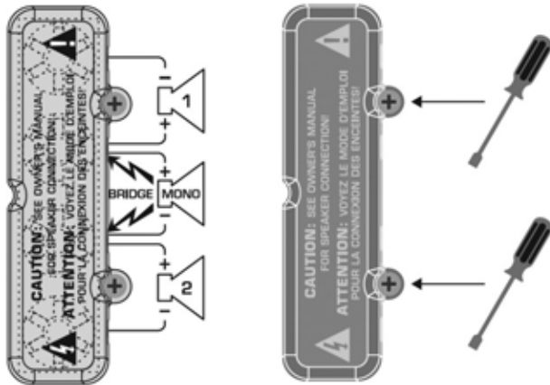
Fig .4.2: Protective plastic covers shielding the binding posts
